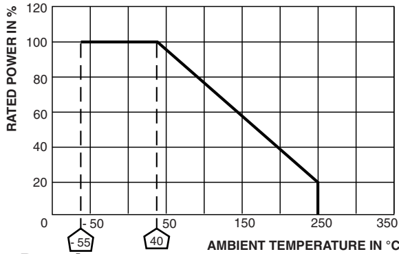
Derating
