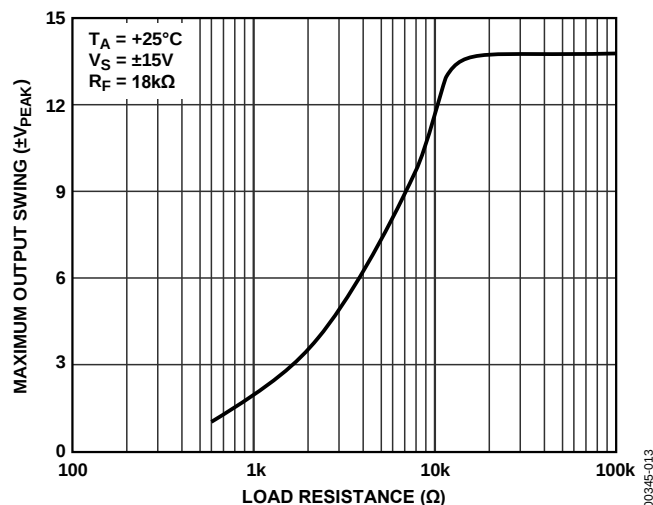
Figure 13. Maximum Output Swing vs. Load Resistance (THD = 1% Max)
