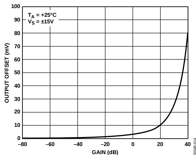
Figure 14. Typical Output Offset vs. Gain
