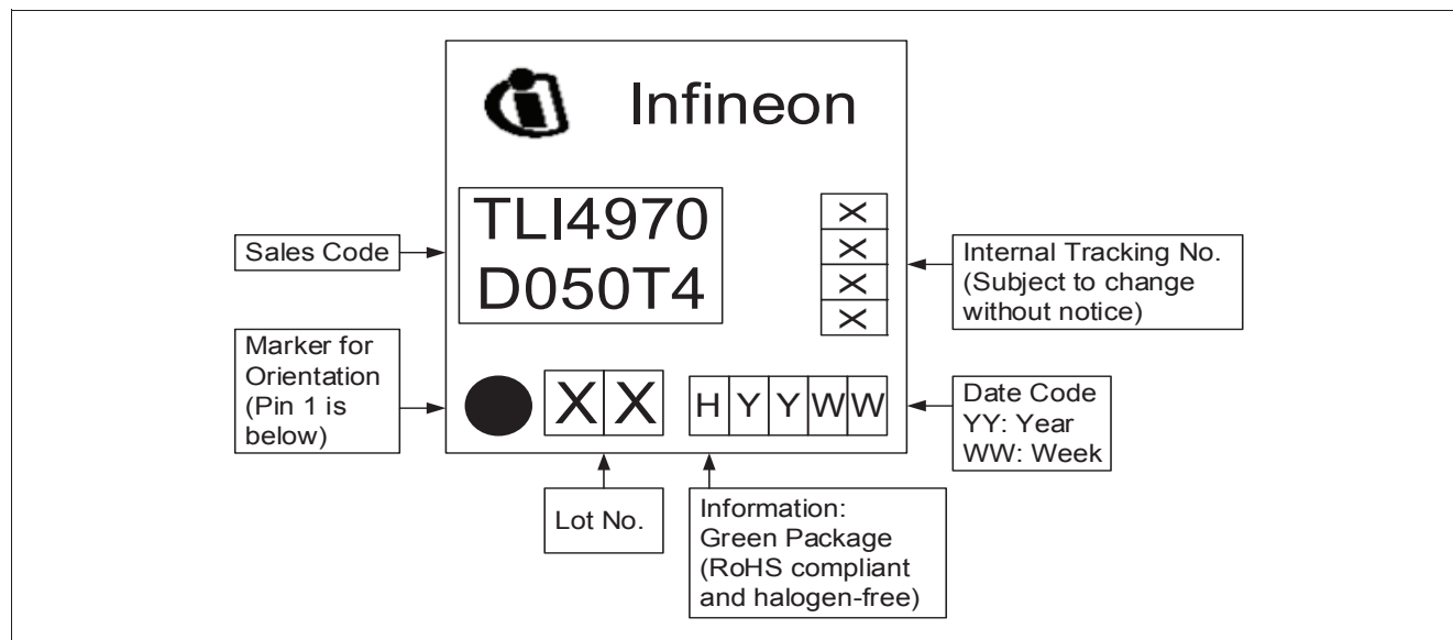
Figure 5-5 Laser marking on the top side
