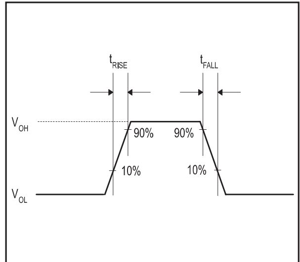
Figure 3. Rise and Fall Times
