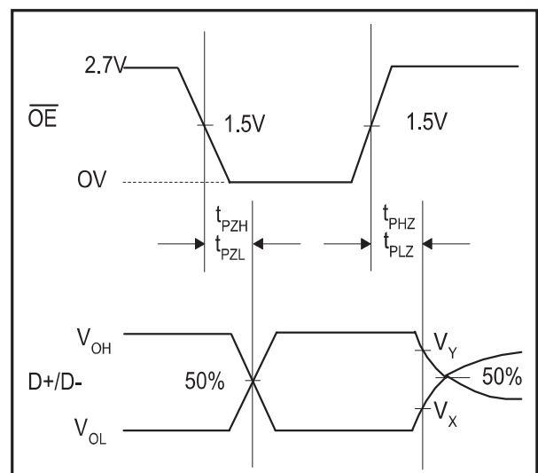
Figure 5. \overline{OE} to D+/D-
