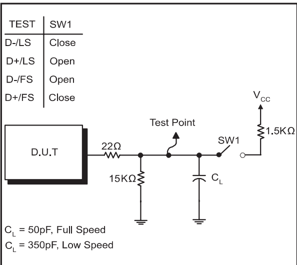
Figure 9. Load for D+/D-
