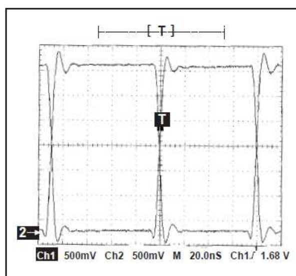
Waveform 2. D+/D- Transmit Mode, full speed
