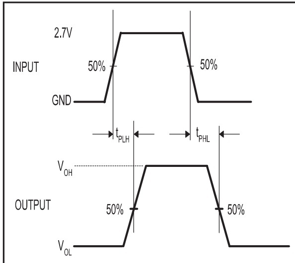
Figure 2. D+/D- to VP/VM or VPO/VMO to D+/D-
