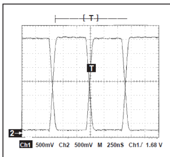
Waveform 1. D+/D- Transmit Mode, low speed
