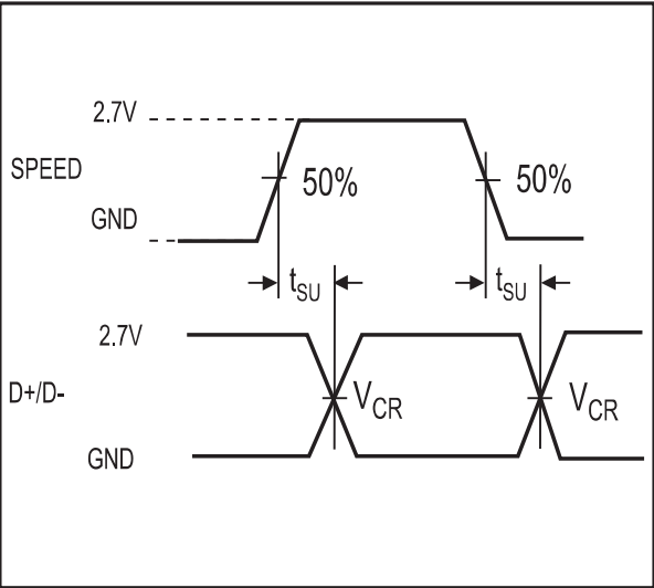
Figure 6. Setup for Speed
