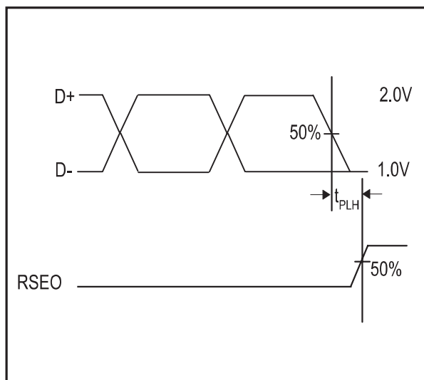
Figure 13. D+/D- to RSEO Delay
