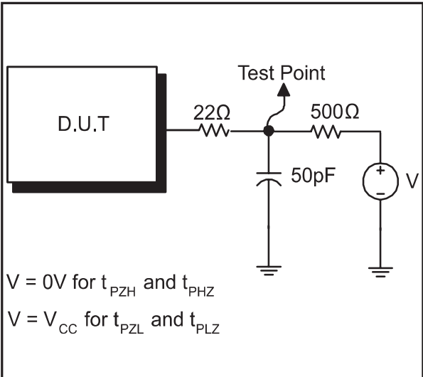
Figure 8. Load for Enable and Disable Times
