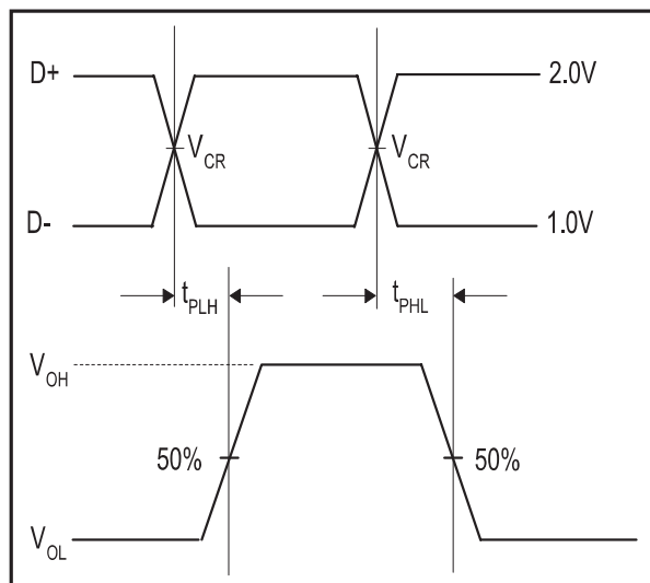
Figure 4. D+/D- to RCV
