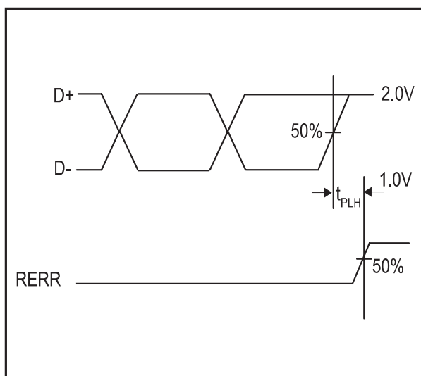
Figure 12. D+/D- to RERR Delay
