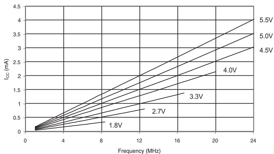
Figure 30-8. Idle supply current vs. frequency (1MHz - 24MHz).
