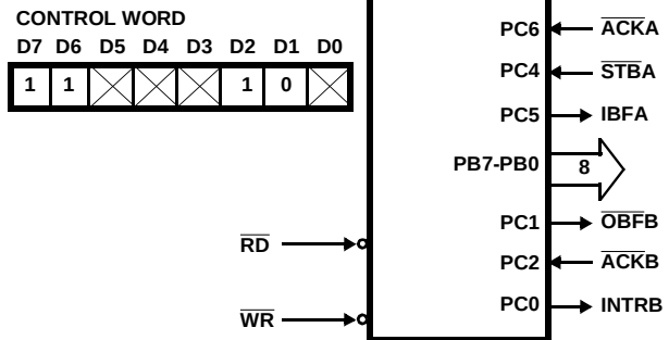
FIGURE 14. MODE 2 COMBINATIONS
