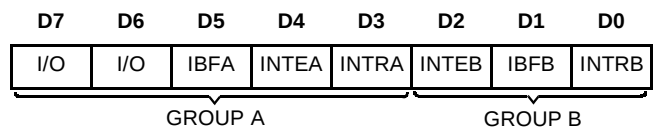
OUTPUT CONFIGURATION
