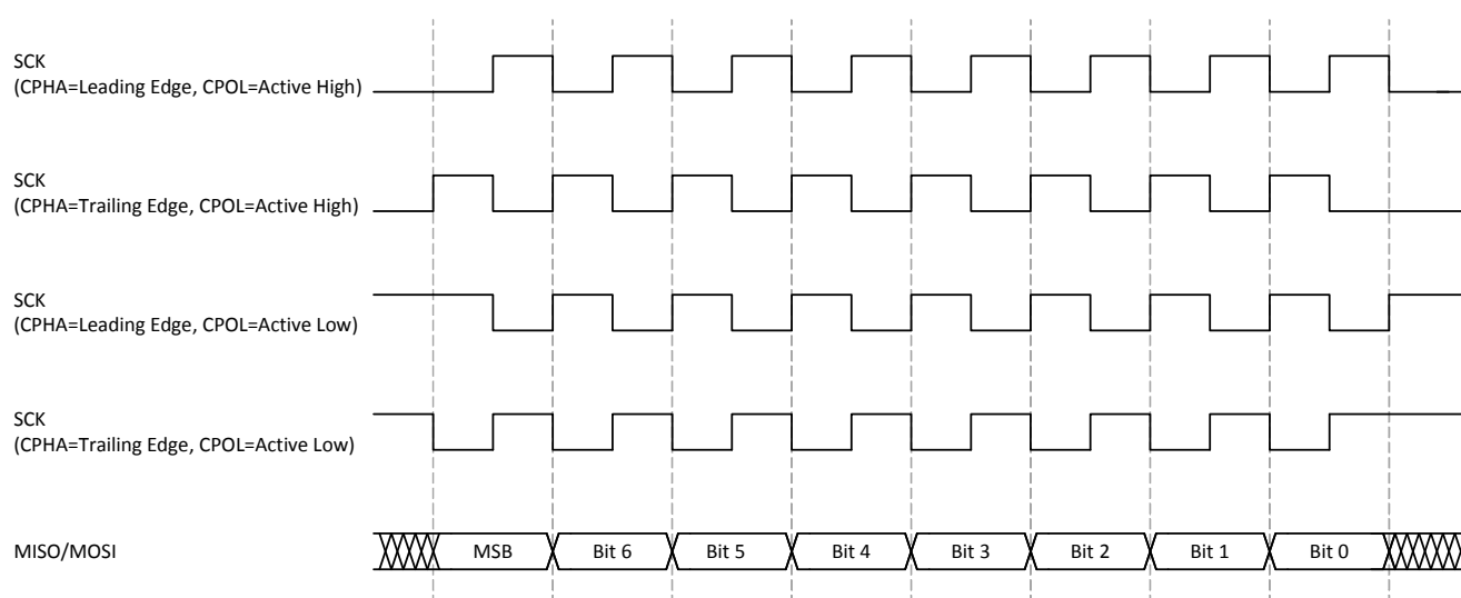
Figure 4. Data/Clock Timing
