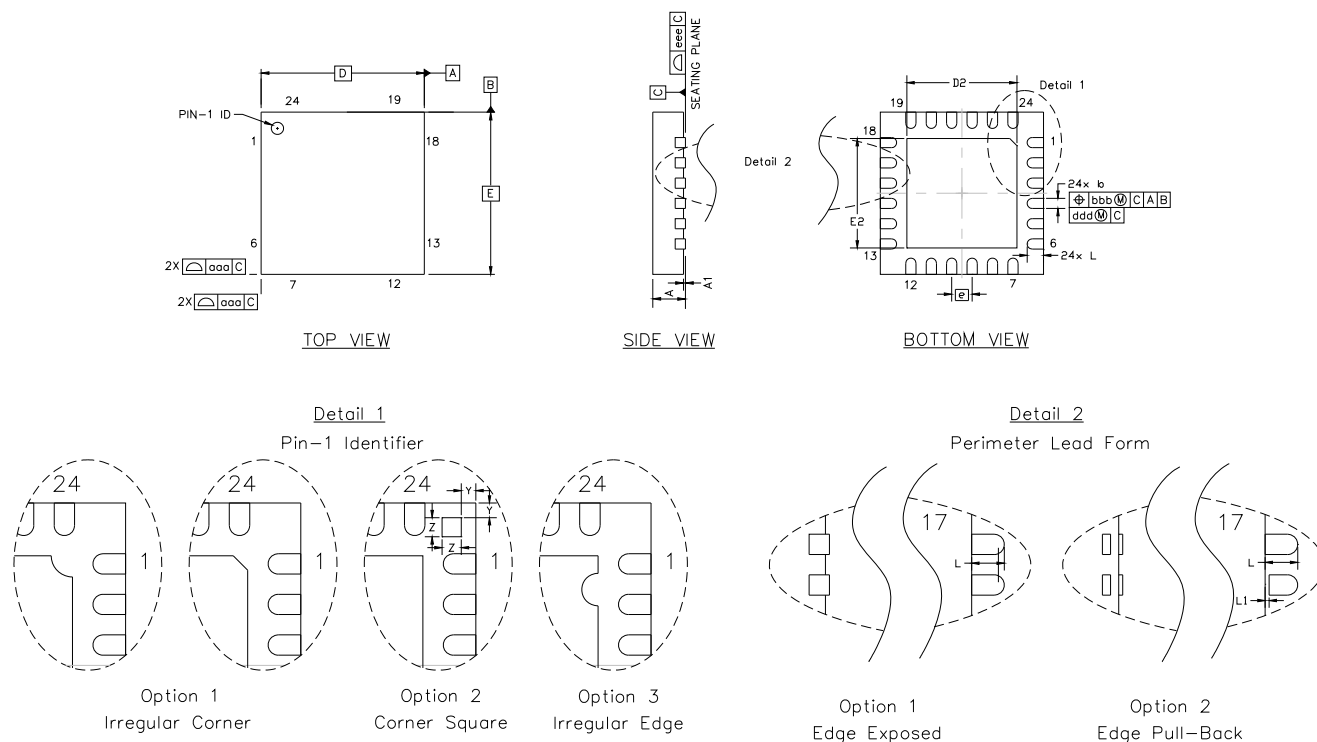
Figure 14. QFN-24 Package Drawing
