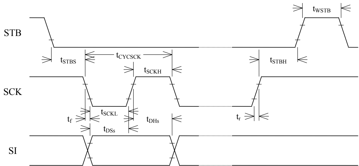
Fig. 5. Synchronous Serial Interface Write Cycle Timing
