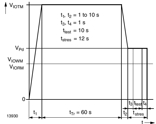
Fig. 2 - Test Pulse Diagram for Sample Test According to DIN EN 60747-5-2 (VDE 0884); IEC60747-5-5
