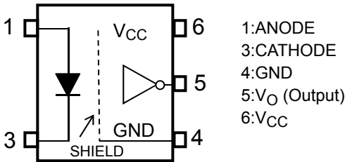
Pin Configuration (Top View)
