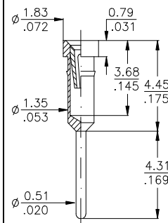
008 long tail terminal
