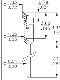
009 extra long tail terminal
