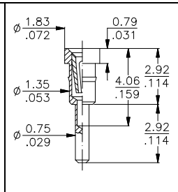
047 Low profile terminal
