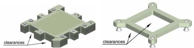
Socket body with clearances
