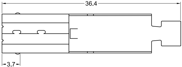
Front Shell
