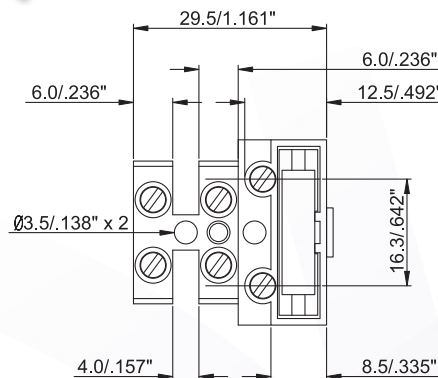
Terminal Block
