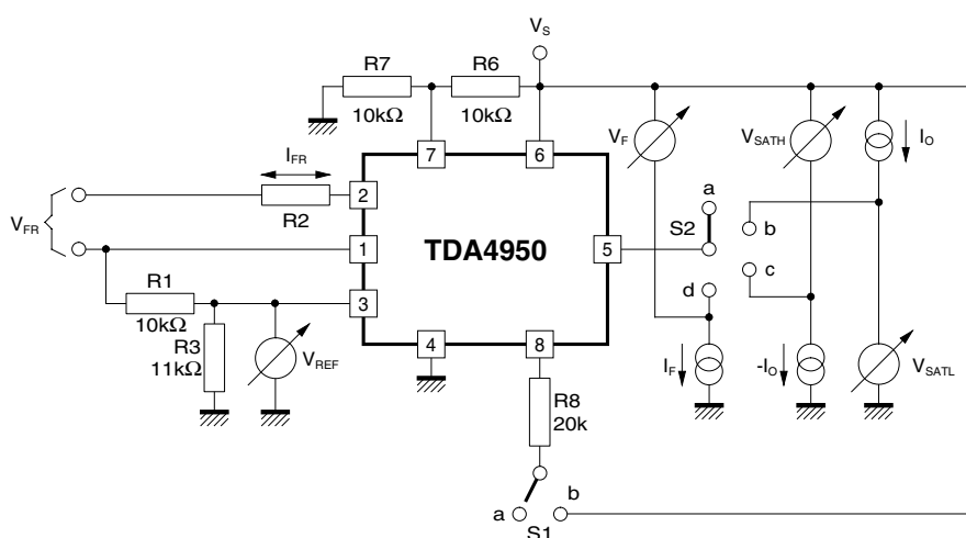
Figure 4. Test Circuit
