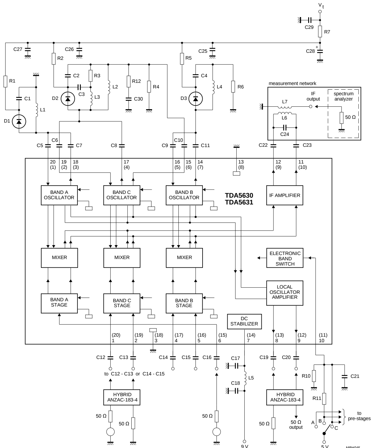
Fig.12 Measurement circuit.
