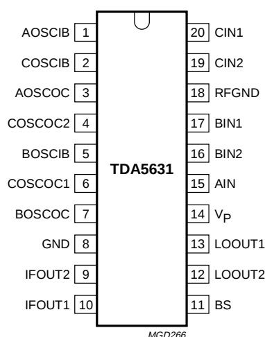
Fig.3 Pin configuration (TDA5631).
