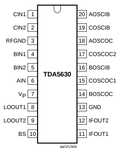
Fig.2 Pin configuration (TDA5630).
