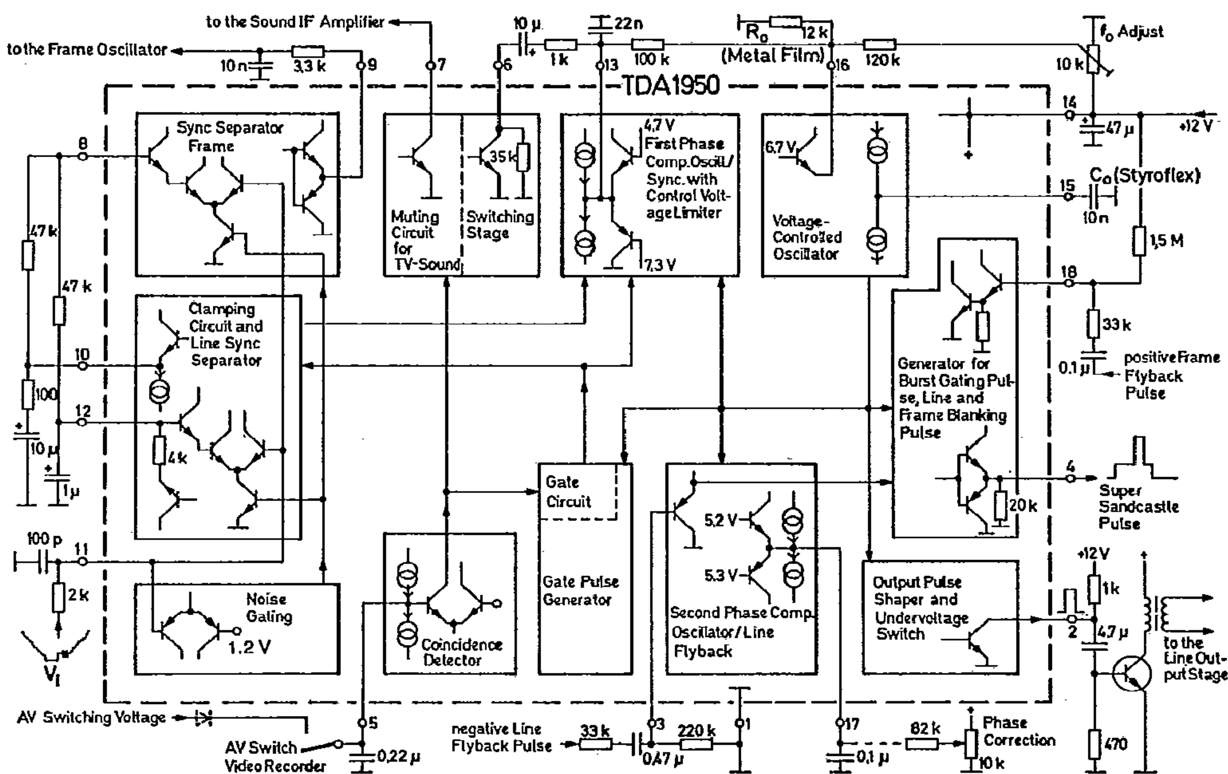
TDA1950 Application Circuit and Block Diagram
