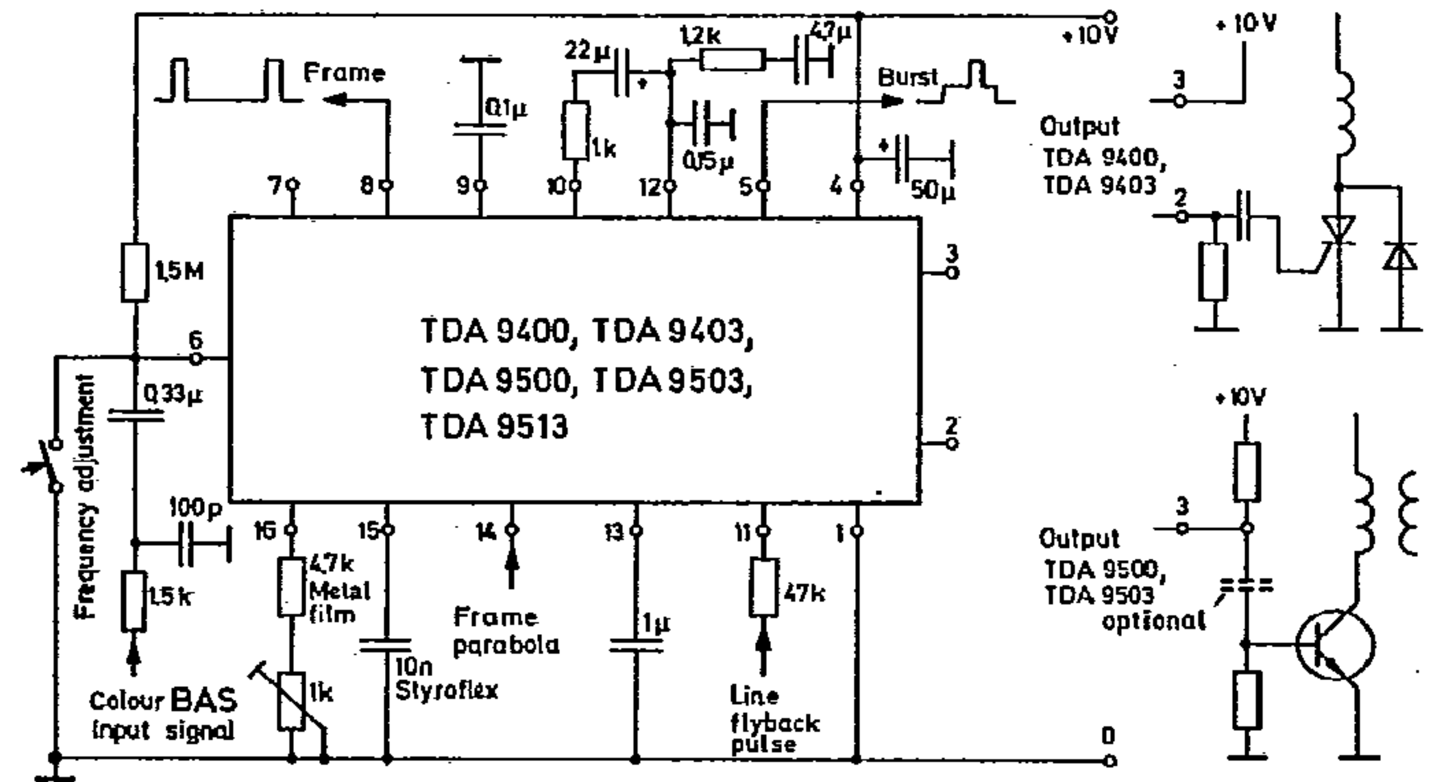
Application Circuit
