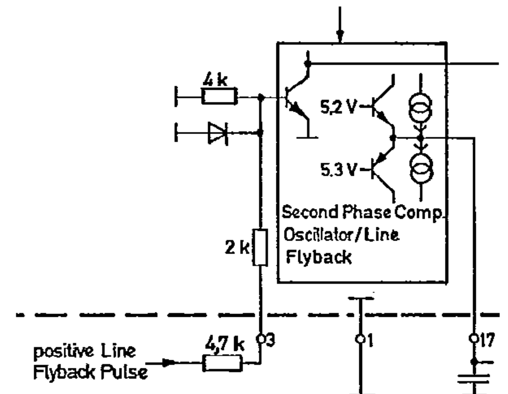
Circuit detail at pin 3 of the types TDA1940 and TDA1940F
