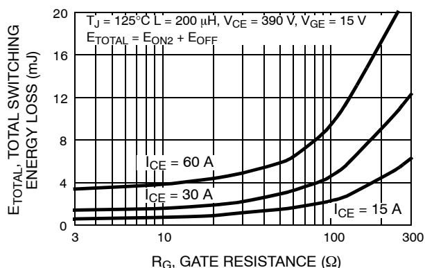
Figure 16. TOTAL SWITCHING LOSS vs. GATE RESISTANCE
