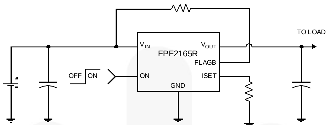
Figure 2. Typical Application
