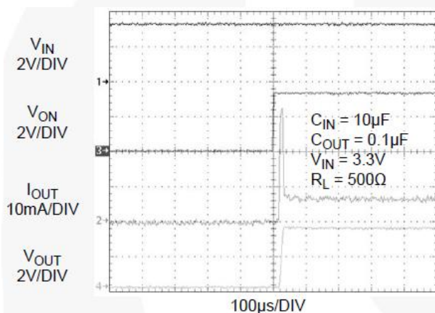
Figure 13. t_{dON} Response
