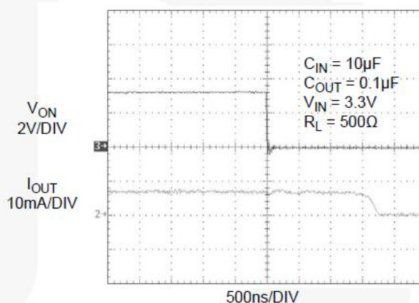
Figure 14. t_{dOFF} Response
