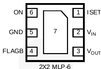
Figure 4. Pin Assignment (Top Through View)
