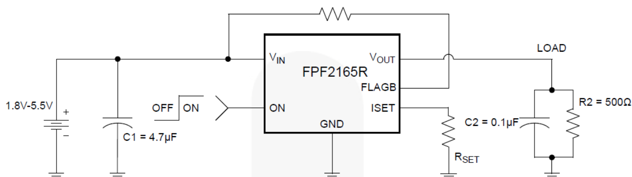
Figure 16. Typical Application
