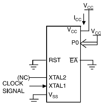
Figure 17-2. I_{CC} Test Condition, Idle Mode
