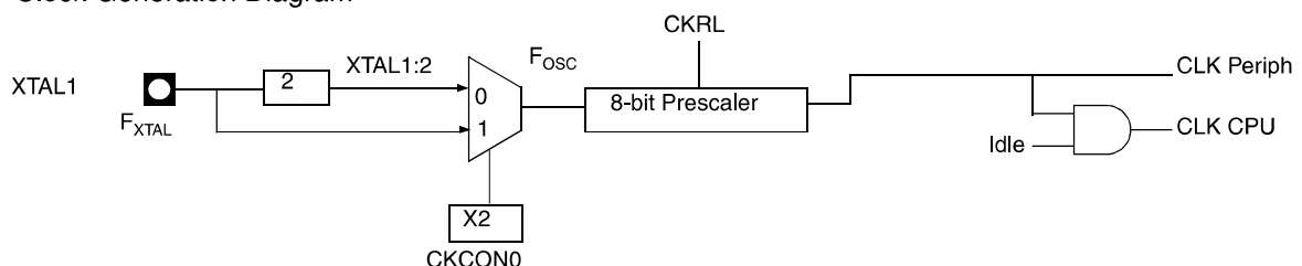
Figure 6-1. Clock Generation Diagram
