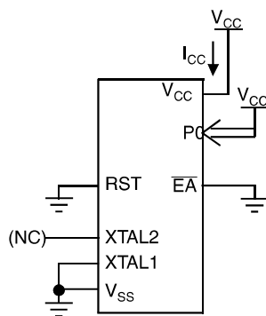
Figure 17-3. I_{CC} Test Condition, Power-down Mode
