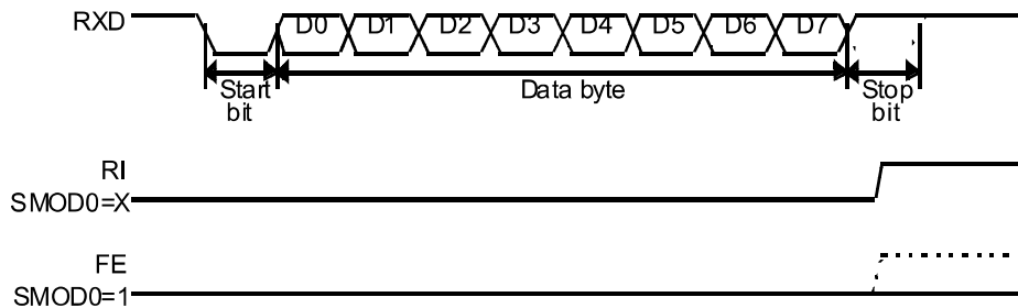
Figure 11-2. UART Timings in Mode 1
