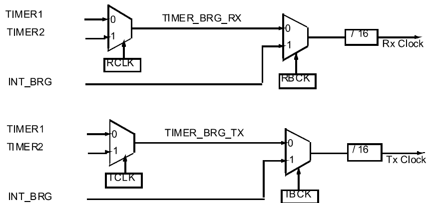
Figure 11-4. Baud Rate selection
