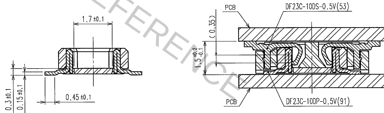
Fig.3 : A-A CROSS SECTION VIEW
