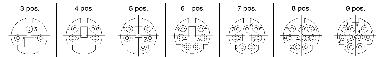
FRONT VIEWS
