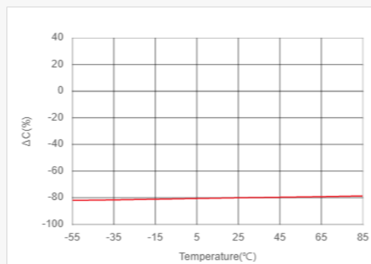
Bias TCC Characteristics LCR meter, 1kHz, 0.5Vrms, 8Vdc
