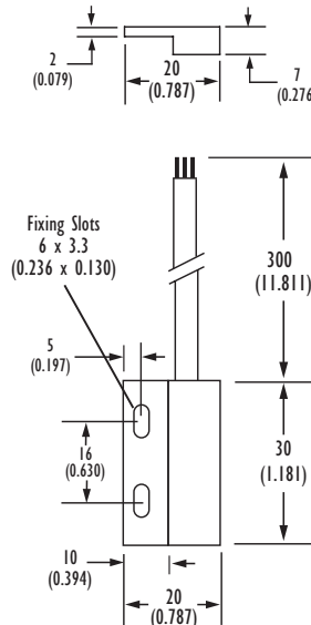
Drawings not to scale All dimensions in mm(inches) nominal
