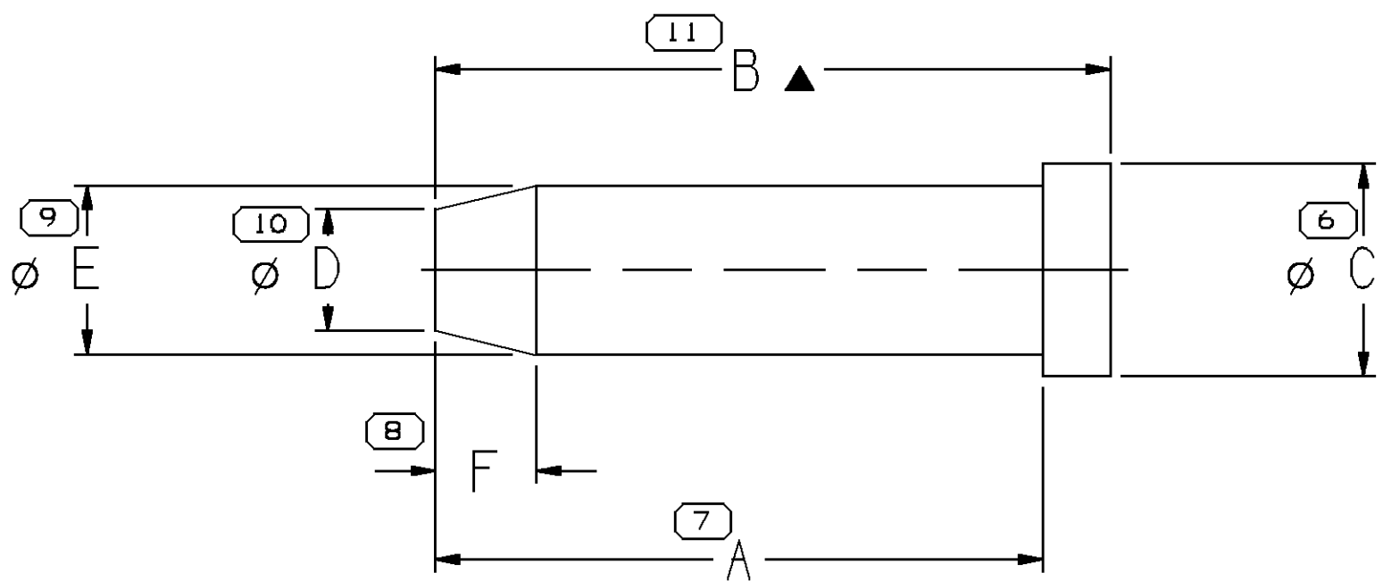
TYPE 102 ALL METRI-PACK PULL TO SEAT -MACHINE INSERTION ONLY-
