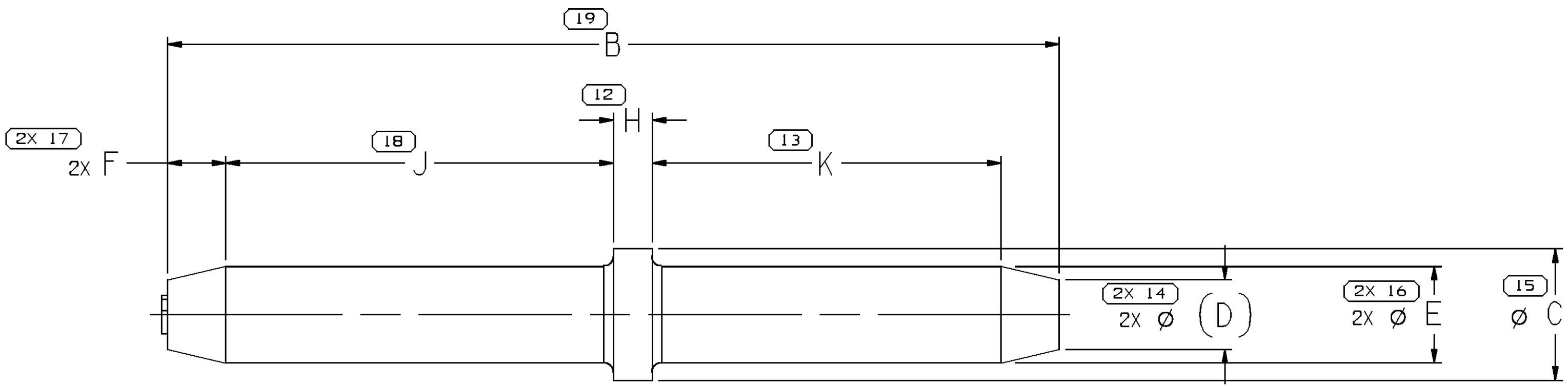
TYPE 101 ALL METRI-PACK PULL TO SEAT -HAND INSERTION ONLY-
