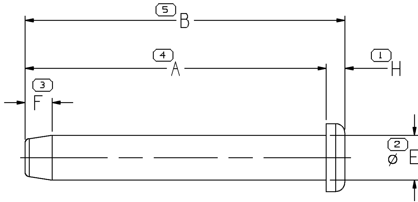
TYPE 103 ALL MICRO-PACK 100W -HAND INSERTION ONLY-
