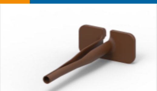
TE Part #0411-354-1605 EXT TOOL, SIZE 16, 16-18 AWG, N, BRN
