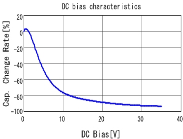
■ GRM188R6YA225KA12 C-DC bias capchange, 25.0degC, AC1.
