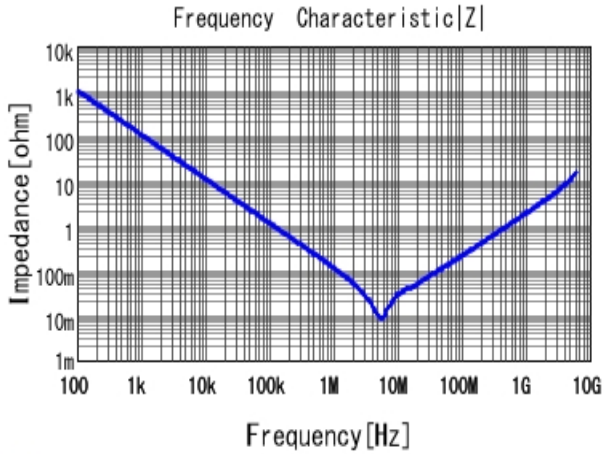
■ GRM188R6YA225KA12 |Z| DCOV, 25degC
