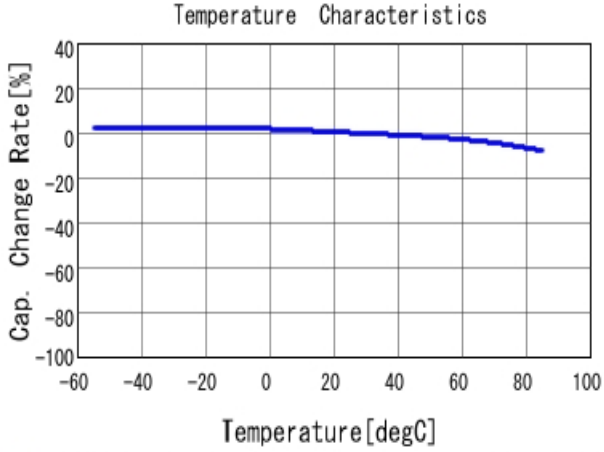
■ GRM188R6YA225KA12 C-Temp. capchange, DC0.0V, AC1.0V rm
