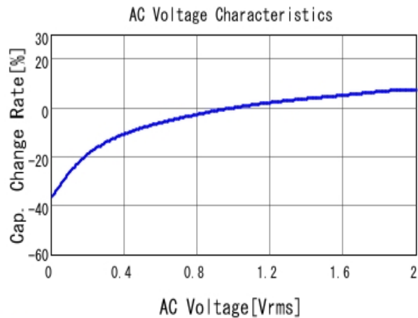
■ GRM188R6YA225KA12 C-AC Voltage capchange, DCOV, 25.0d
