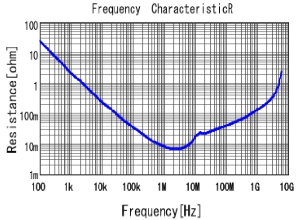
■ GRM188R6YA225KA12 R DCOV, 25degC
