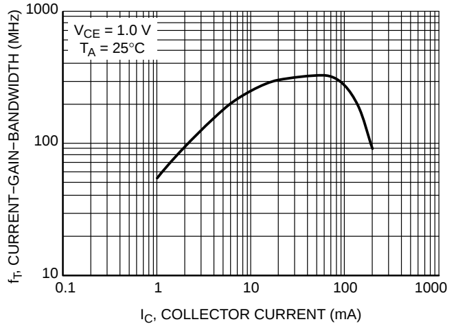
Figure 21. Current-Gain-Bandwidth Product
