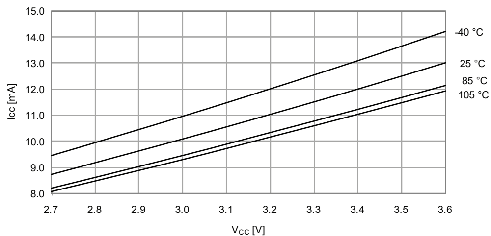
Figure 33-359. Active mode supply current vs. V_{CC} .
