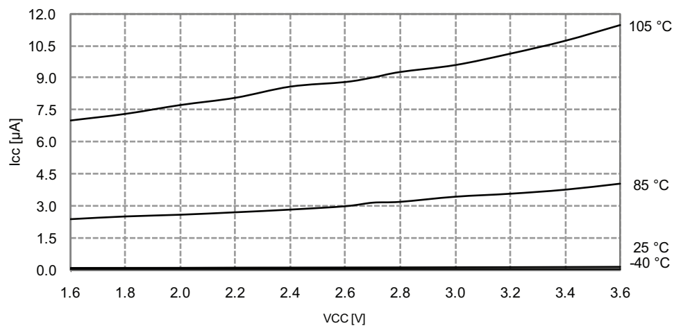
Figure 33-297. Power-down mode supply current vs. V_{CC} . All functions disabled.
