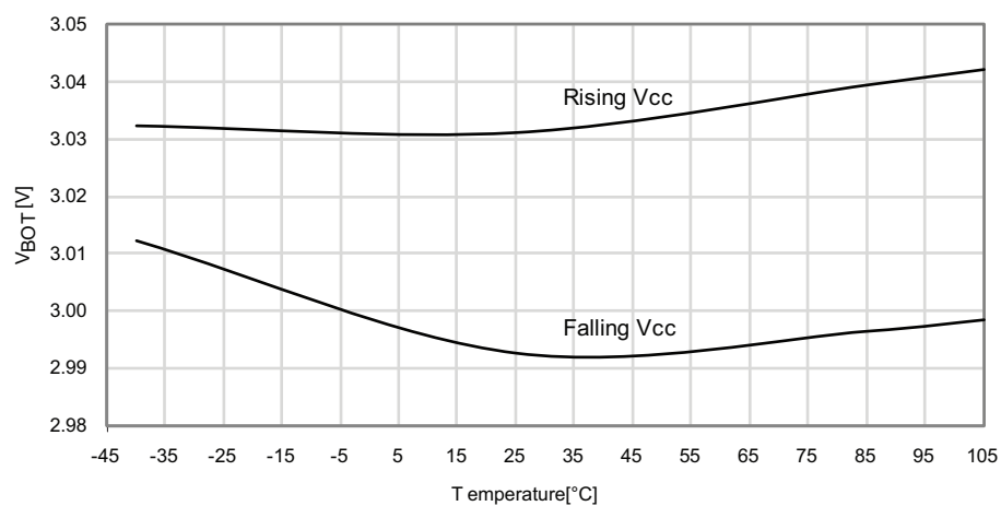
Figure 33-189. BOD thresholds vs. temperature.
