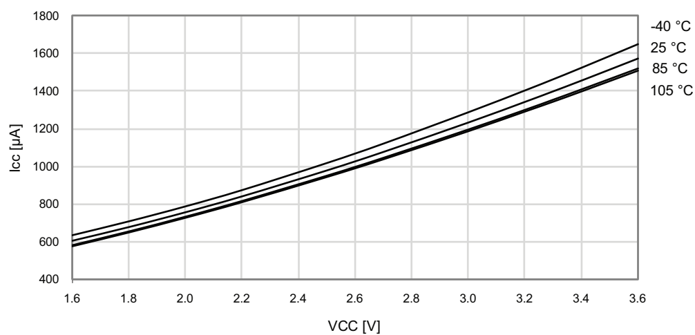
Figure 33-156. Idle mode current vs. V_{CC} .
