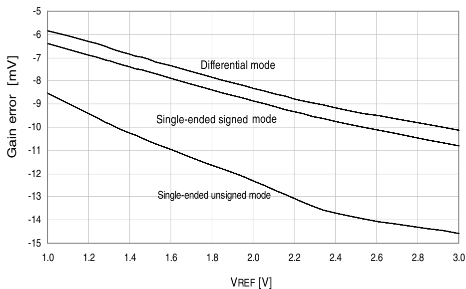
Figure 33-248.Gain error vs. V_{REF} . T = 25^{\circ}\text{C} , V_{CC} = 3.6\text{V} , ADC sample rate = 300kps.
