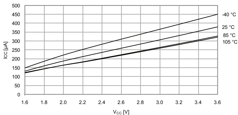
Figure 33-355. Active mode supply current vs. V_{CC} .
