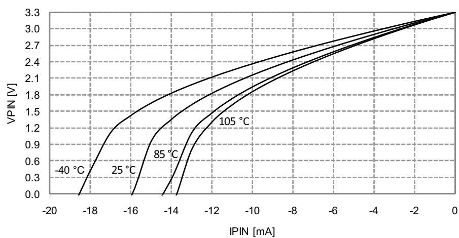
Figure 33-235. I/O pin output voltage vs. source current.
