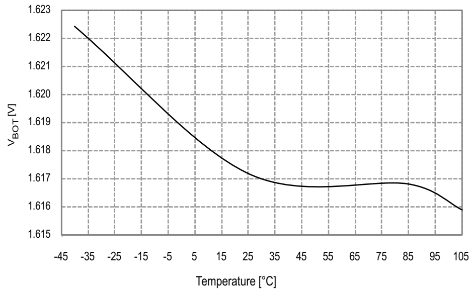
Figure 33-118. BOD thresholds vs. temperature. BOD level = 1.6V.
