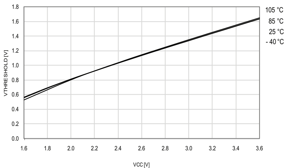
Figure 33-53. Reset pin input threshold voltage vs. V_{CC} .
