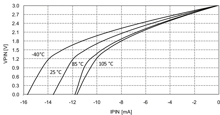
Figure 33-234. I/O pin output voltage vs. source current.
