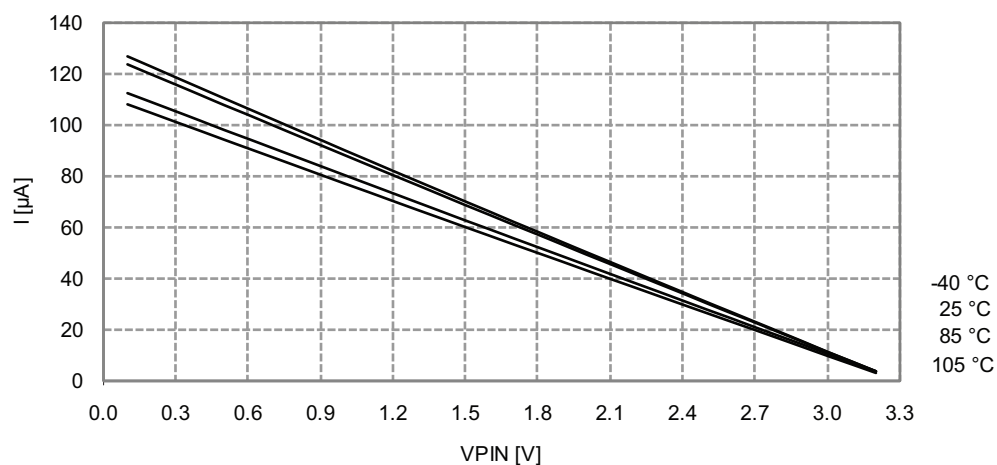
Figure 33-232. I/O pin pull-up resistor current vs. input voltage.
