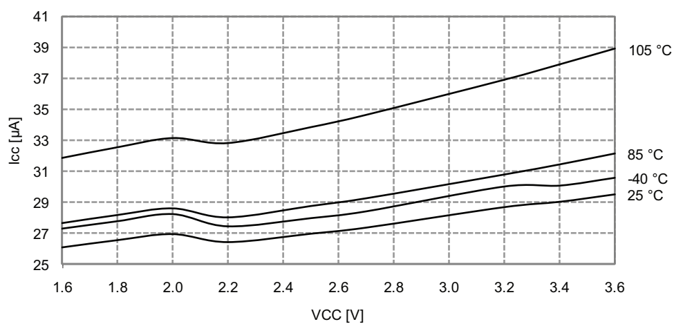
Figure 33-292. Idle mode supply current vs. V_{CC} .
