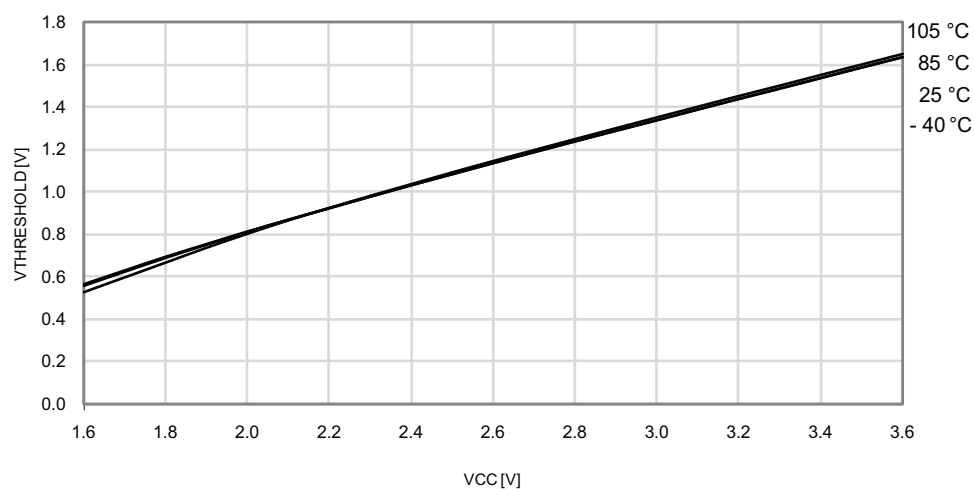
Figure 33-334. Reset pin input threshold voltage vs. V_{CC} .
