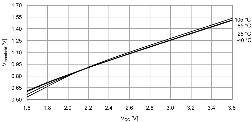
Figure 33-380. I/O pin input threshold voltage vs. V_{CC} . V_{IL} I/O pin read as “0”.
