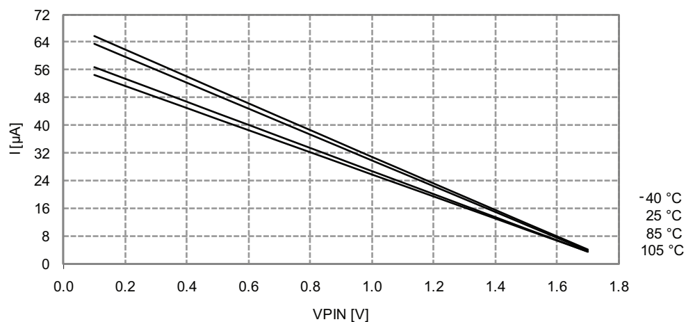
Figure 33-230. I/O pin pull-up resistor current vs. input voltage.
