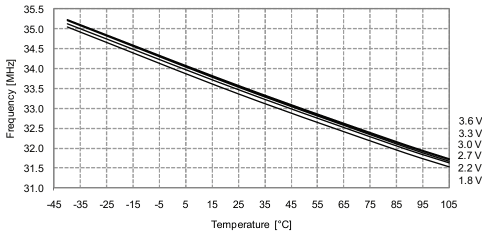
Figure 33-341. 32MHz internal oscillator frequency vs. temperature. DPLL disabled.
