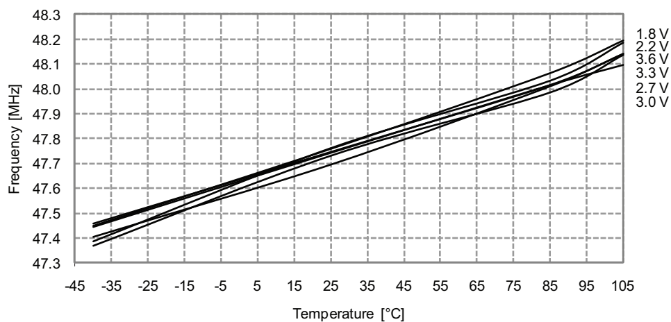
Figure 33-279. 48MHz internal oscillator frequency vs. temperature. DFLL enabled, from the 32.768kHz internal oscillator.
