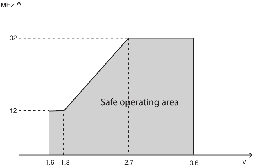
Figure 32-1. Maximum frequency vs. V CC .
