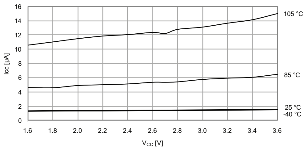
Figure 33-368. Power-down mode supply current vs. V_{CC} . Watchdog and sampled BOD enabled.
