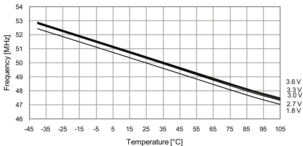
Figure 33-208. 48MHz internal oscillator frequency vs. temperature.
