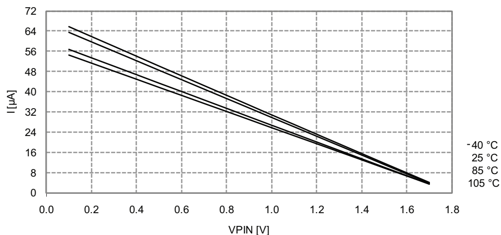
Figure 33-300. I/O pin pull-up resistor current vs. input voltage.
