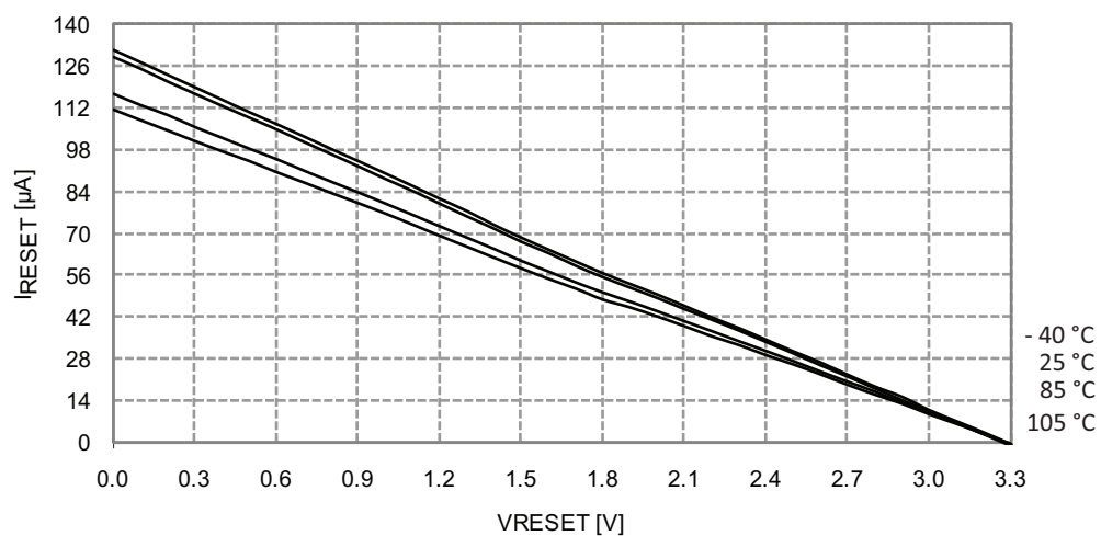
Figure 33-263. Reset pin pull-up resistor current vs. reset pin voltage.
