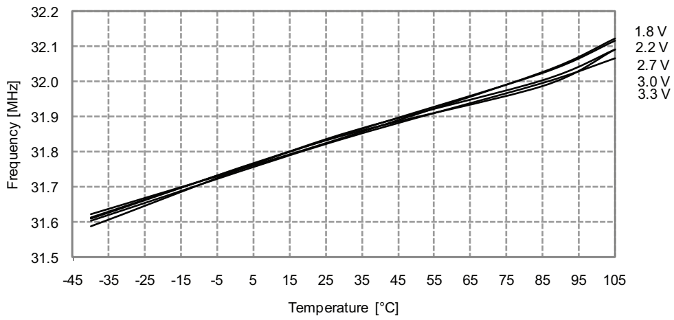
Figure 33-272. 32MHz internal oscillator frequency vs. temperature. DFLL enabled, from the 32.768kHz internal oscillator.
