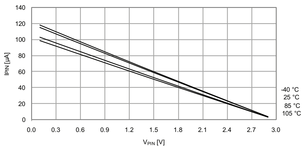
Figure 33-371. I/O pin pull-up resistor current vs. input voltage.
