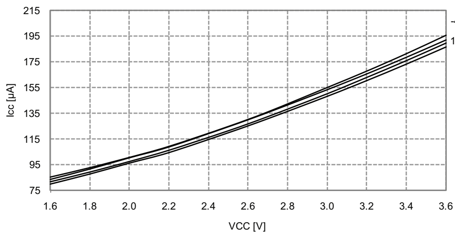
Figure 33-294. Idle mode supply current vs. V_{CC} .
