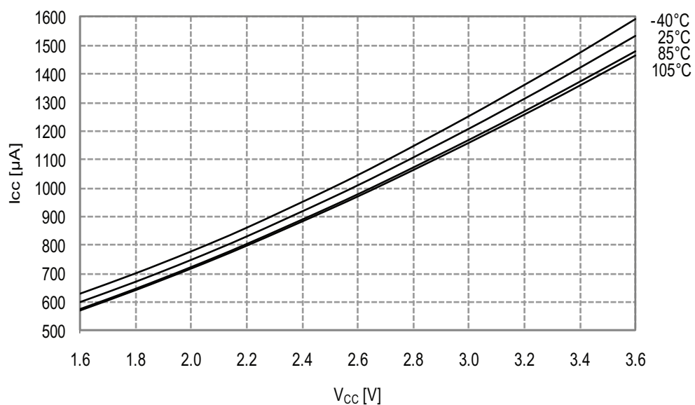
Figure 33-85. Idle mode current vs. V_{CC} .
