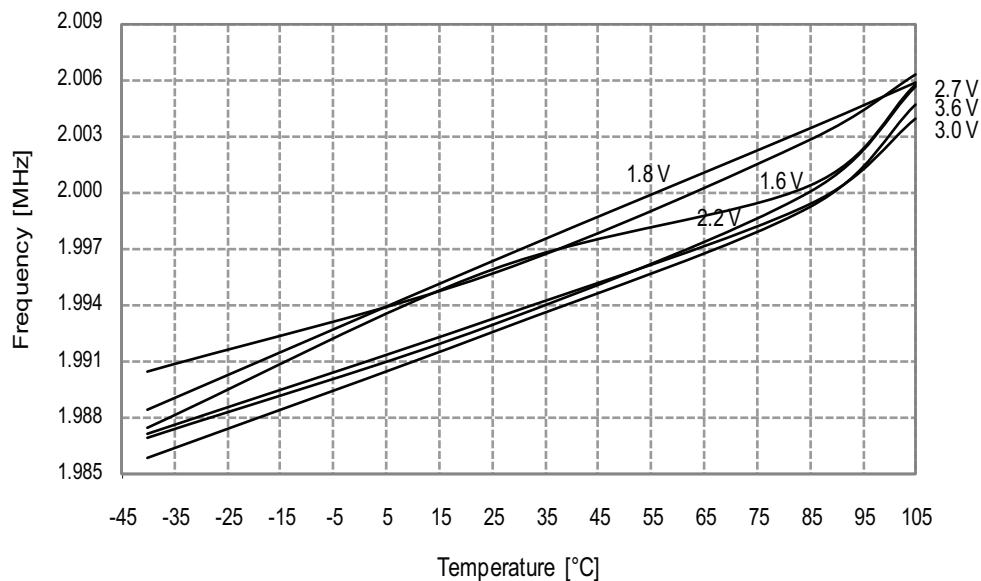
Figure 33-129. 2MHz internal oscillator frequency vs. temperature.
