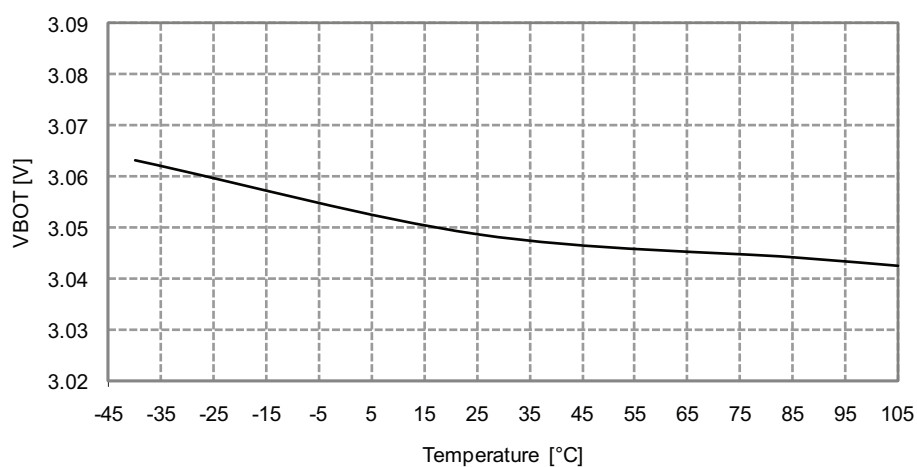
Figure 33-329. BOD thresholds vs. temperature.
