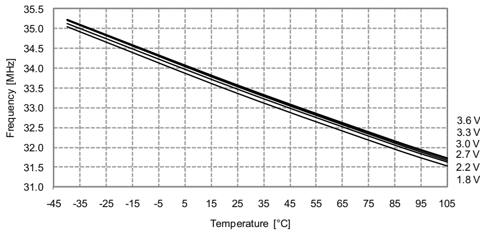
Figure 33-271. 32MHz internal oscillator frequency vs. temperature. DFLL disabled.
