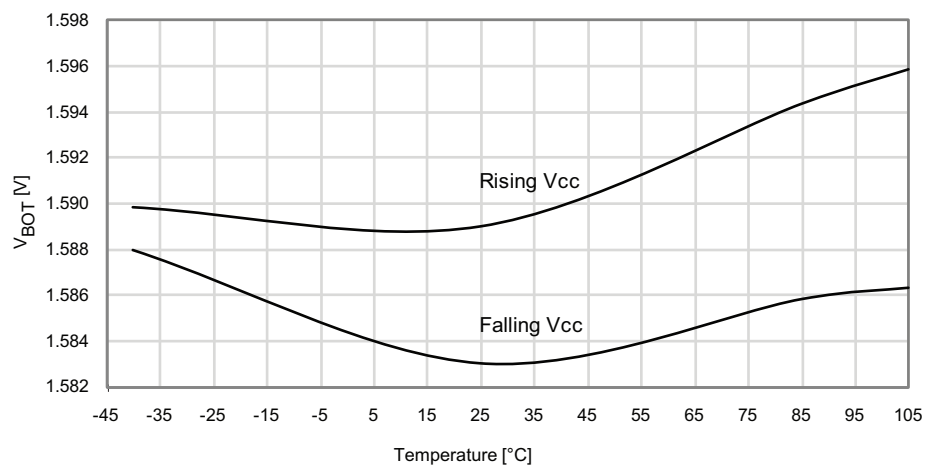
Figure 33-188. BOD thresholds vs. temperature.
