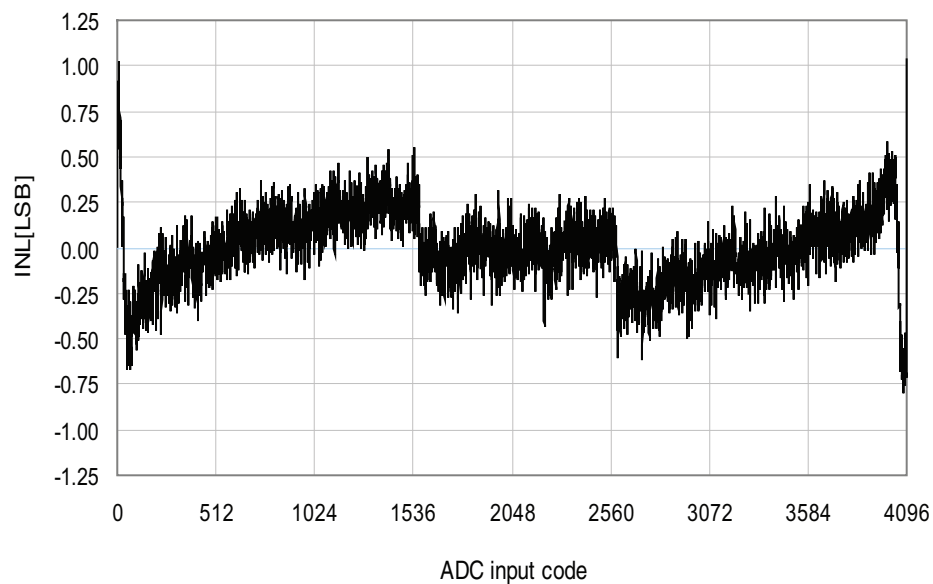
Figure 33-244. INL error vs. input code.
