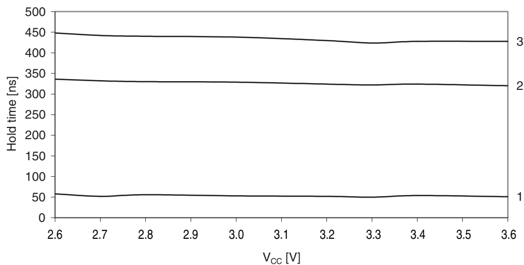
Figure 33-351. SDA hold time vs. supply voltage.
