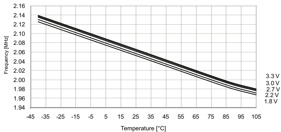
Figure 33-198. 2MHz internal oscillator frequency vs. temperature.
