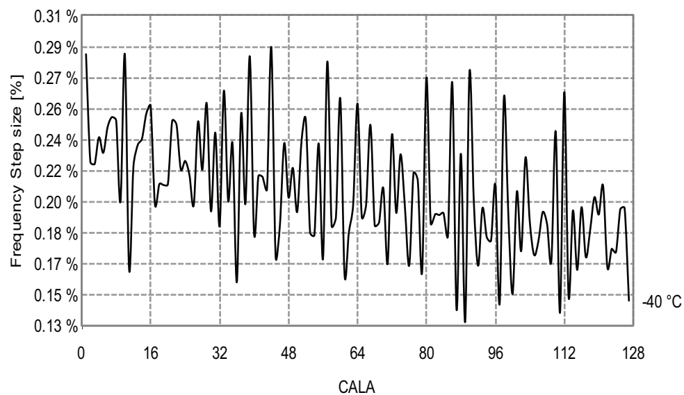
Figure 33-133. 32MHz internal oscillator CALA calibration step size.
