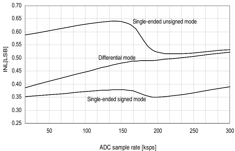
Figure 33-103. INL error vs. sample rate.
