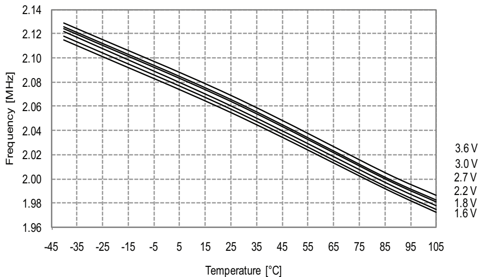
Figure 33-129. 2MHz internal oscillator frequency vs. temperature.
