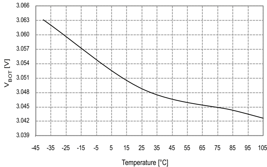
Figure 33-119. BOD thresholds vs. temperature. BOD level = 3.0V.
