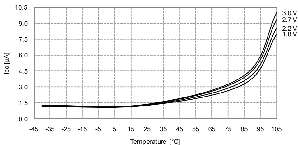
Figure 33-229. Power-down mode supply current vs. Temperature.
