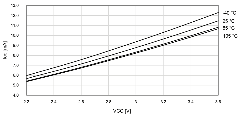
Figure 33-149. Active mode supply current vs. V_{CC} .
