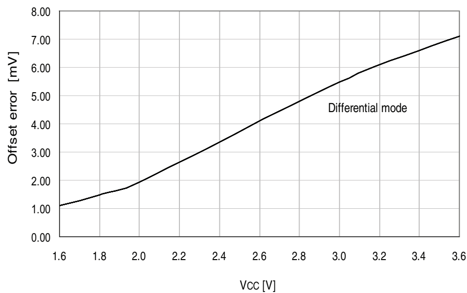
Figure 33-322. Offset error vs. V_{CC} .
