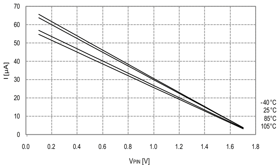
Figure 33-91. I/O pin pull-up resistor current vs. input voltage.
