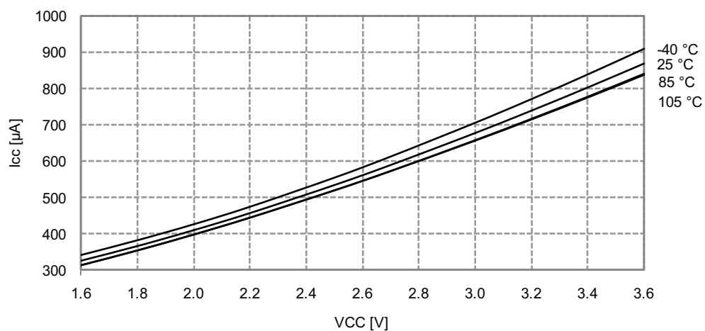
Figure 33-295. Idle mode supply current vs. V_{CC} .
