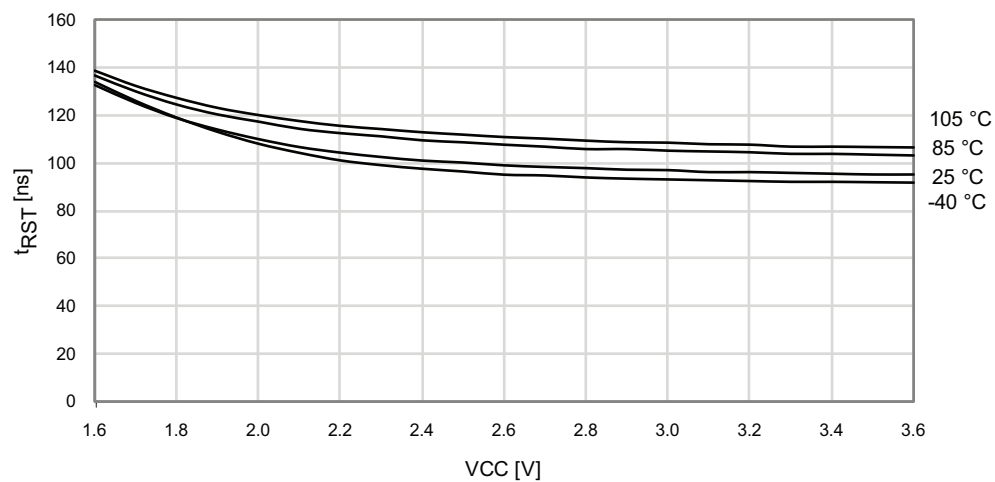
Figure 33-190. Minimum Reset pin pulse width vs. V CC .
