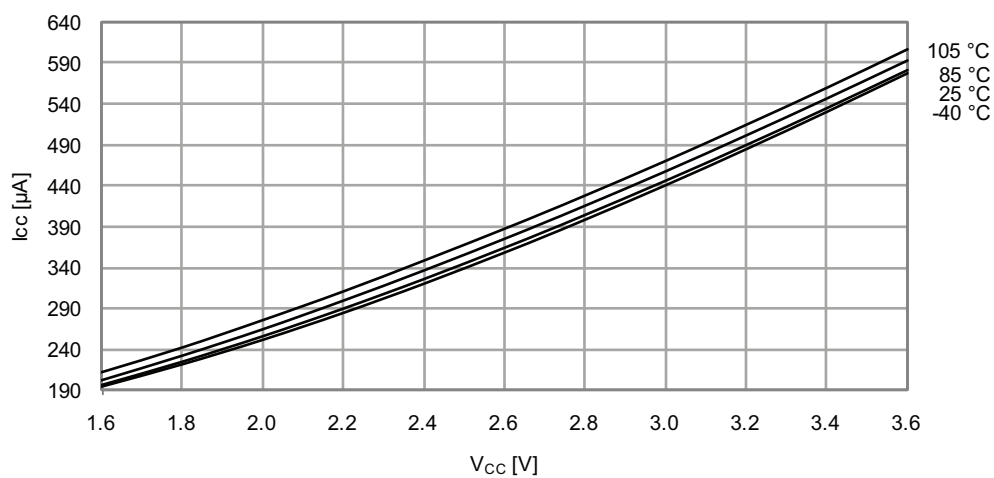
Figure 33-364. Idle mode supply current vs. V_{CC} .
