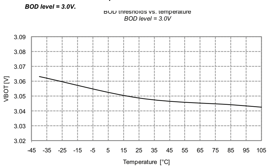
Figure 33-259. BOD thresholds vs. temperature.
