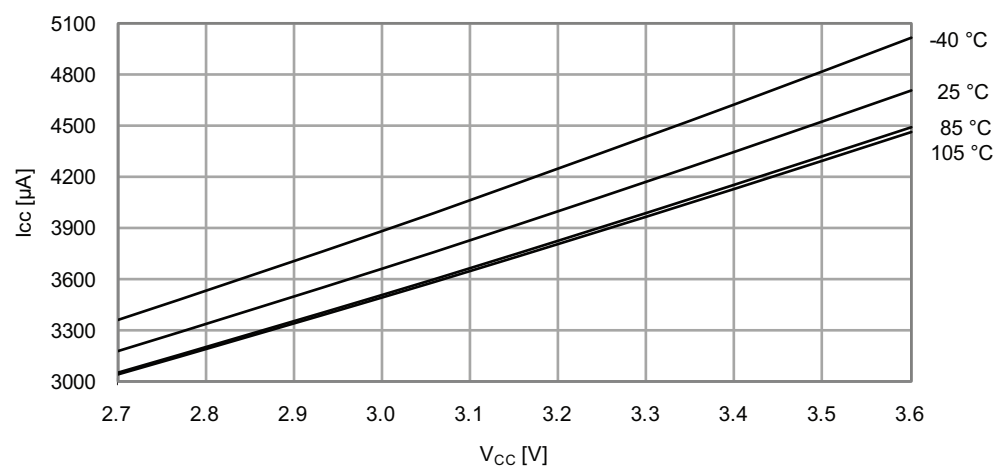
Figure 33-366. Idle mode current vs. V_{CC} .
