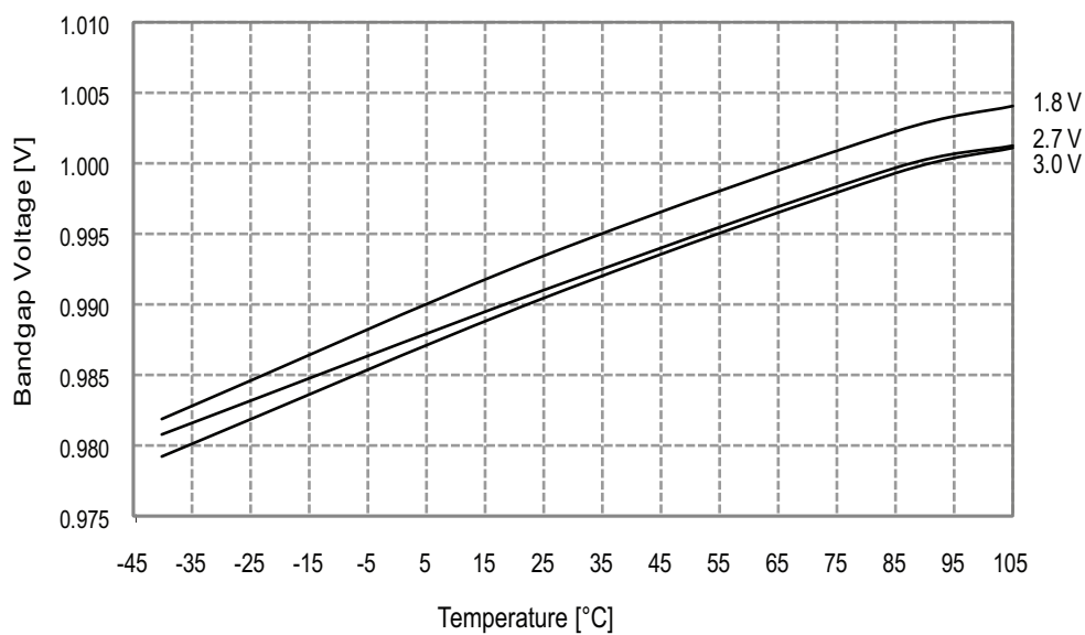
Figure 33-117. ADC Internal 1.0V reference vs. temperature.
