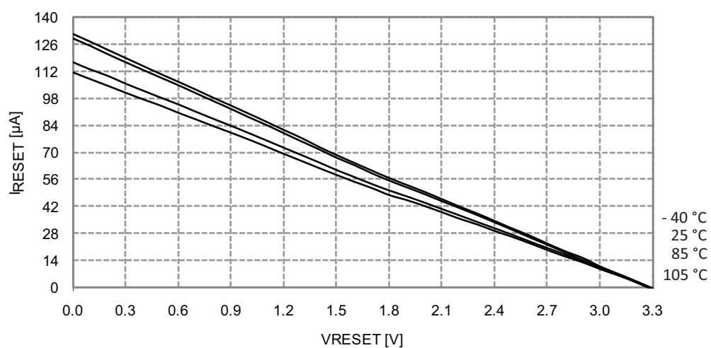
Figure 33-333. Reset pin pull-up resistor current vs. reset pin voltage.
