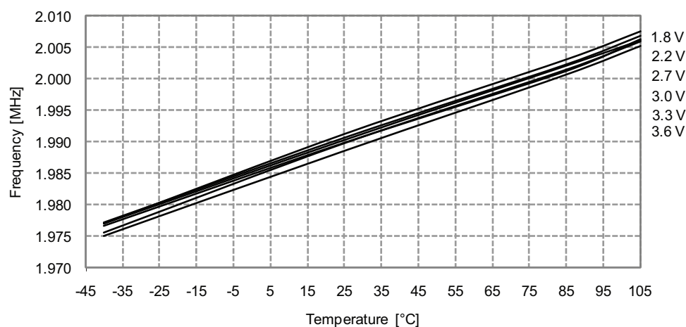
Figure 33-339. 2MHz internal oscillator frequency vs. temperature. DPLL enabled, from the 32.768kHz internal oscillator.
