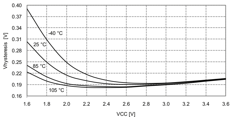
Figure 33-241. I/O pin input hysteresis vs. V_{CC} .
