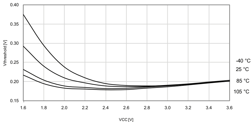
Figure 33-171. I/O pin input hysteresis vs. V_{CC} .
