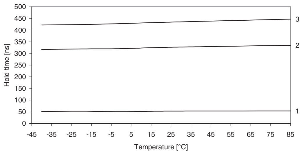
Figure 33-350. SDA hold time vs. temperature.
