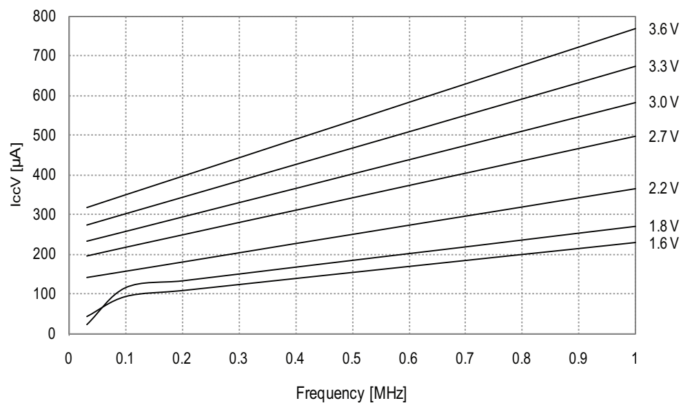
Figure 33-73. Active supply current vs. frequency.
