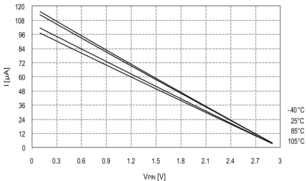
Figure 33-91. I/O pin pull-up resistor current vs. input voltage.
