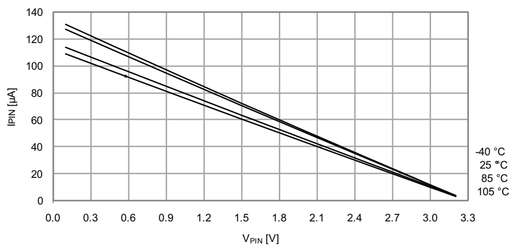
Figure 33-372. I/O pin pull-up resistor current vs. input voltage.
