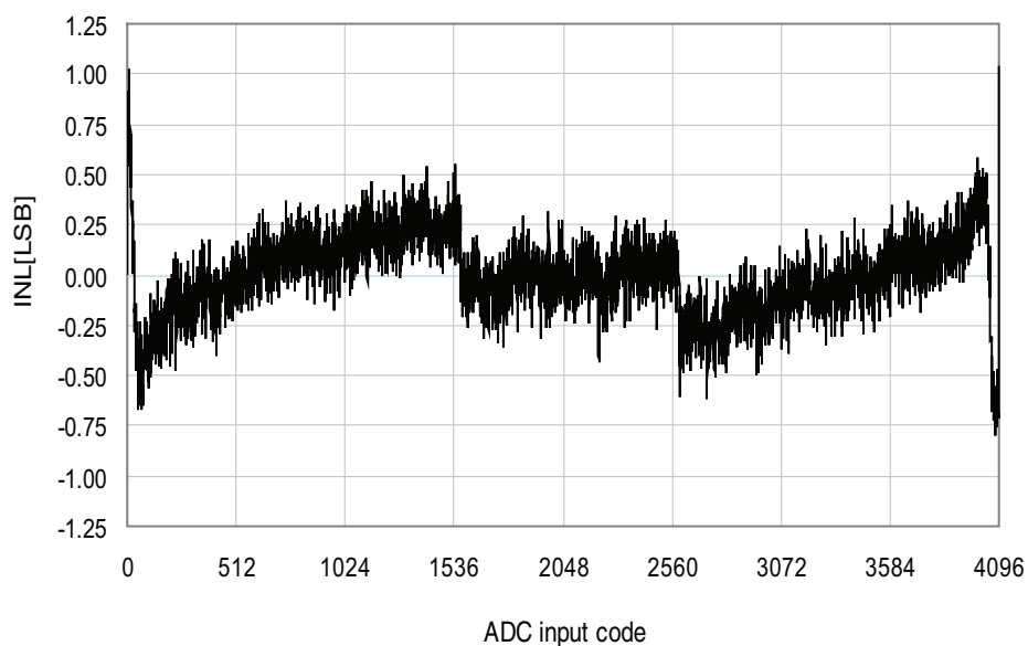
Figure 33-174. INL error vs. input code.
