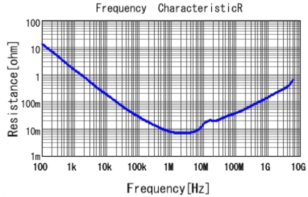
GRT155C81C225KE13 R DCOV, 25degC
