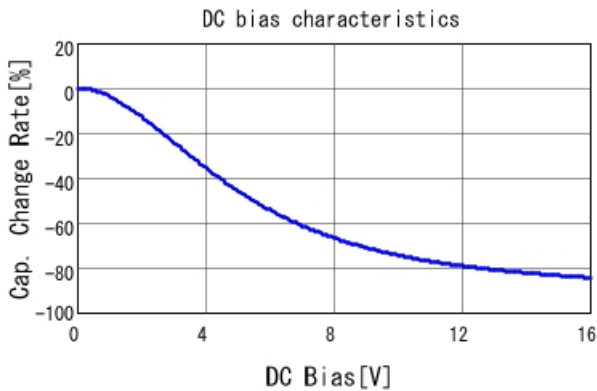
GRT155C81C225KE13 C-DC bias capchange, 25.0degC, A
