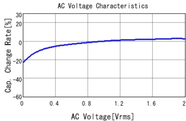
GRT155C81C225KE13 C-AC Voltage capchange, DCOV, 25
