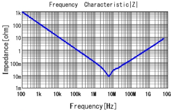
GRT155C81C225KE13 |Z| DCOV, 25degC
