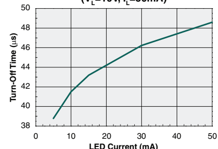
Typical Turn-Off Time vs. LED Forward Current ( V_L=10\text{V} , I_L=50\text{mA} )
