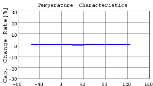
■ GCM1555C1H6R8DA16 C-Temp. capchange, DCOV, 1
