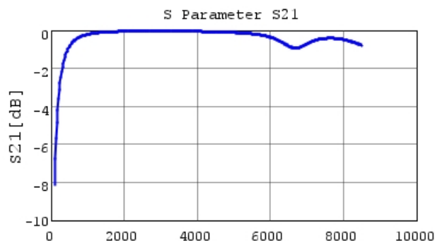
■ GCM1555C1H6R8DA16 S21 DCOV, 25degC
