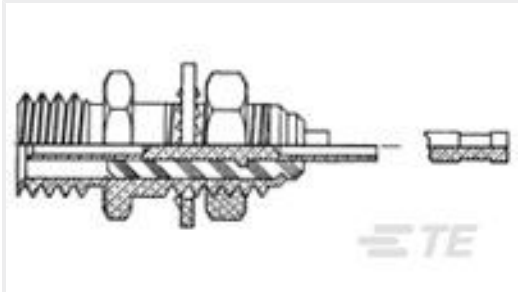
TE Part #1-1532006-1 141-0002-0001=RCPT,FTMTW/TURR
