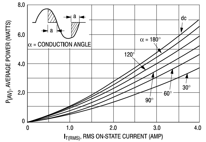
Figure 4. Power Dissipation
