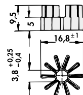
KK 1895 TO 18 48 K/W
