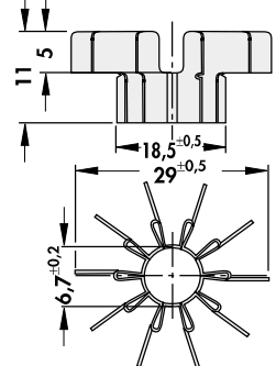
KK 511 TO 5 33 K/W
