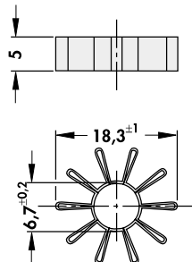
KK 505 TO 5 60 K/W
