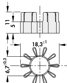
KK 5095 S TO 5 46 K/W
