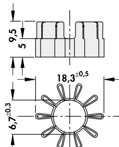
KK 5095 TO 5 48 K/W
