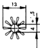
KK 184 TO 18 65 K/W
